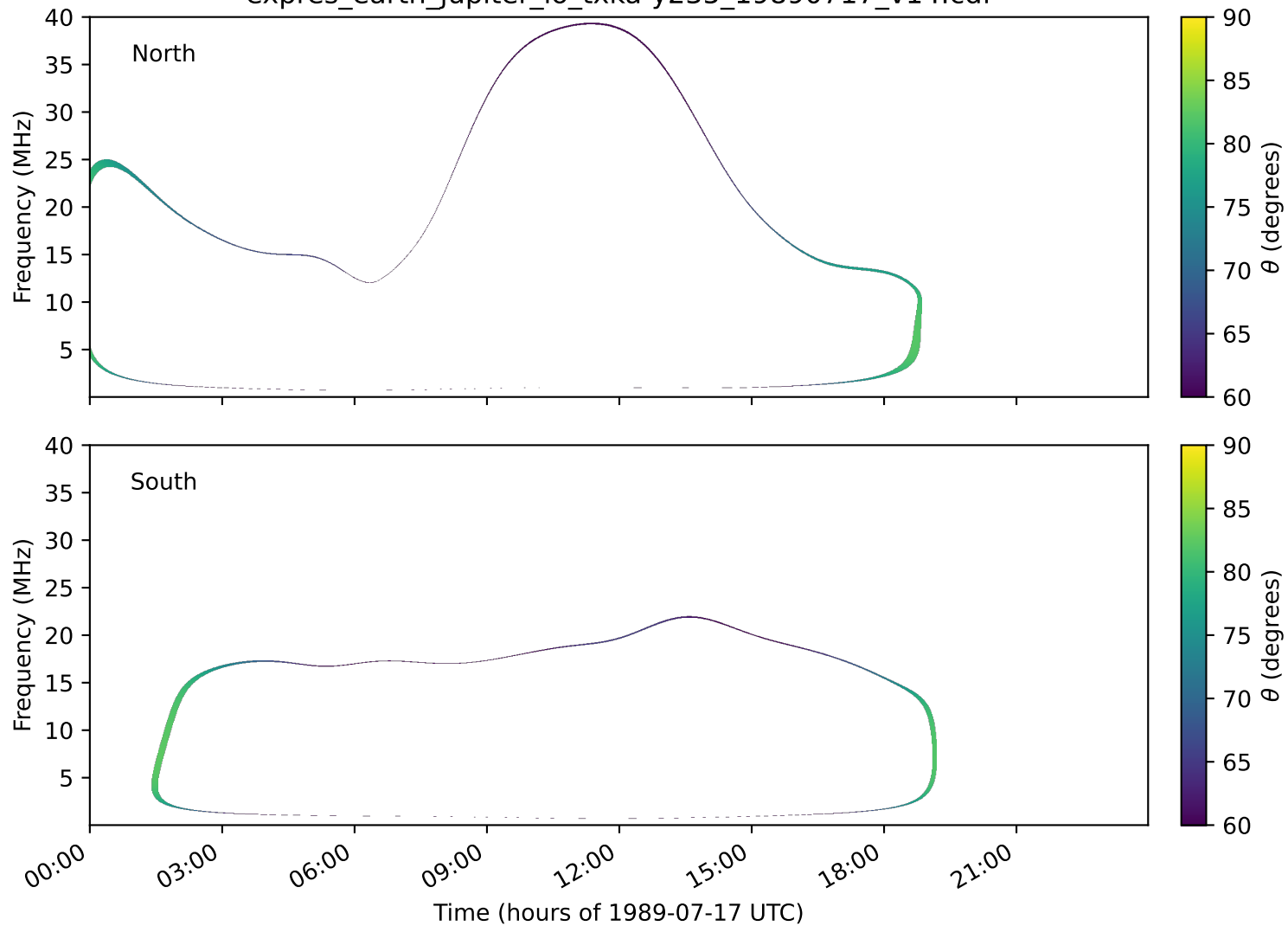
expres_earth_jupiter_io_txka-y235_19890717_v14.cdf
