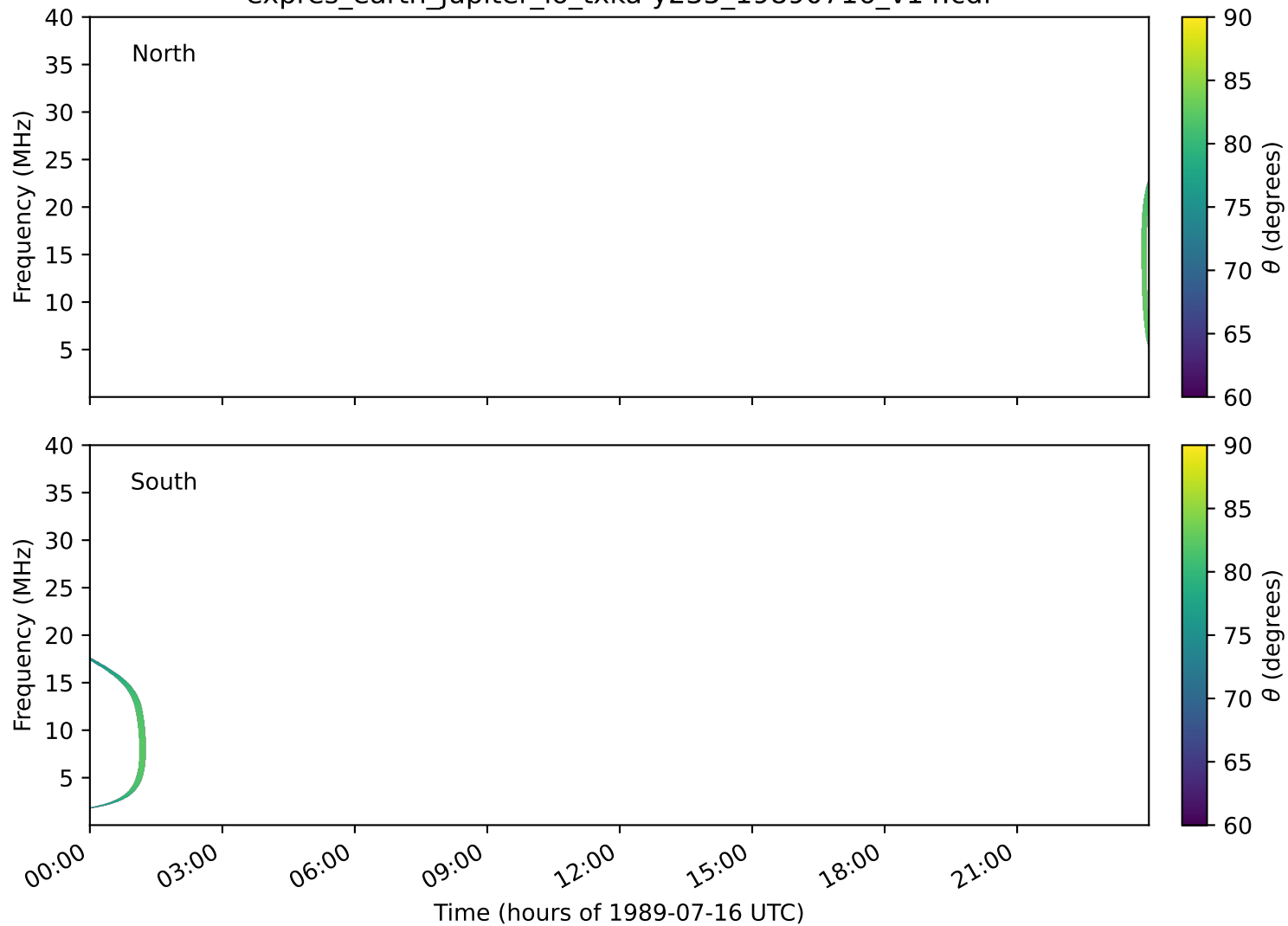
expres_earth_jupiter_io_txka-y235_19890716_v14.cdf
