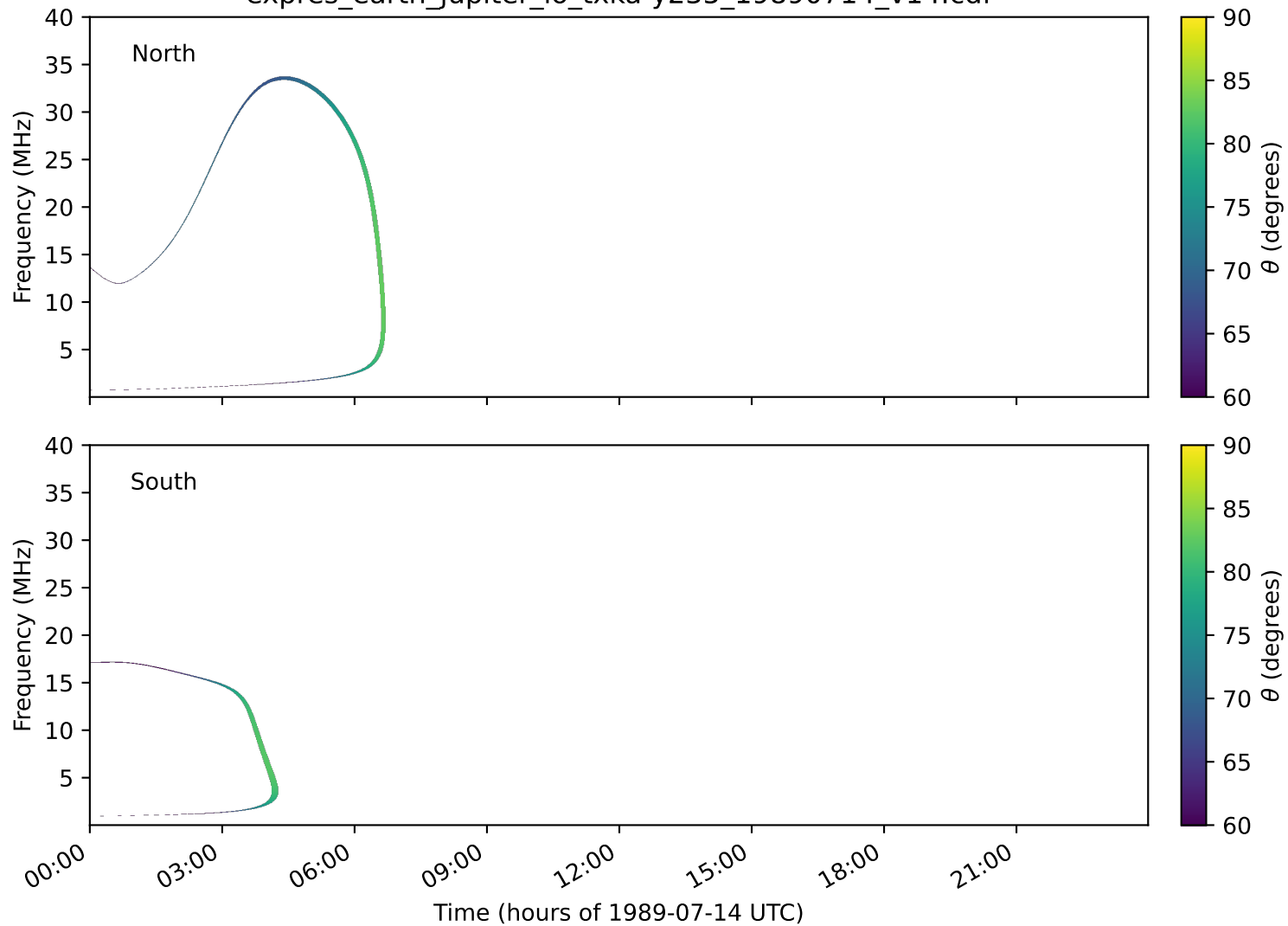
expres_earth_jupiter_io_txka-y235_19890714_v14.cdf
