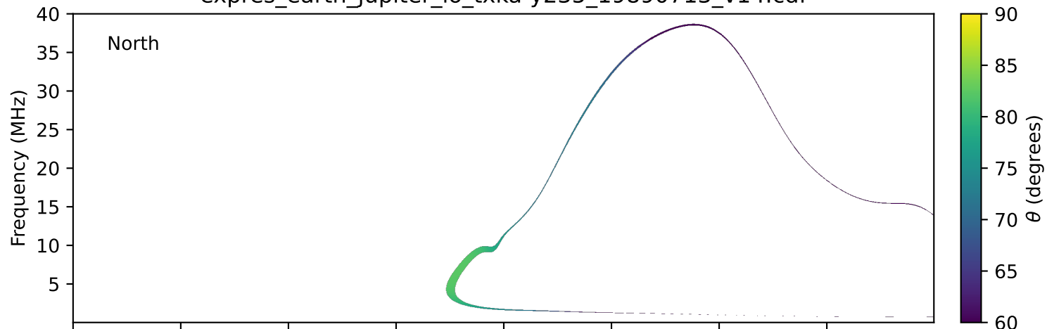
expres_earth_jupiter_io_txka-y235_19890713_v14.cdf
