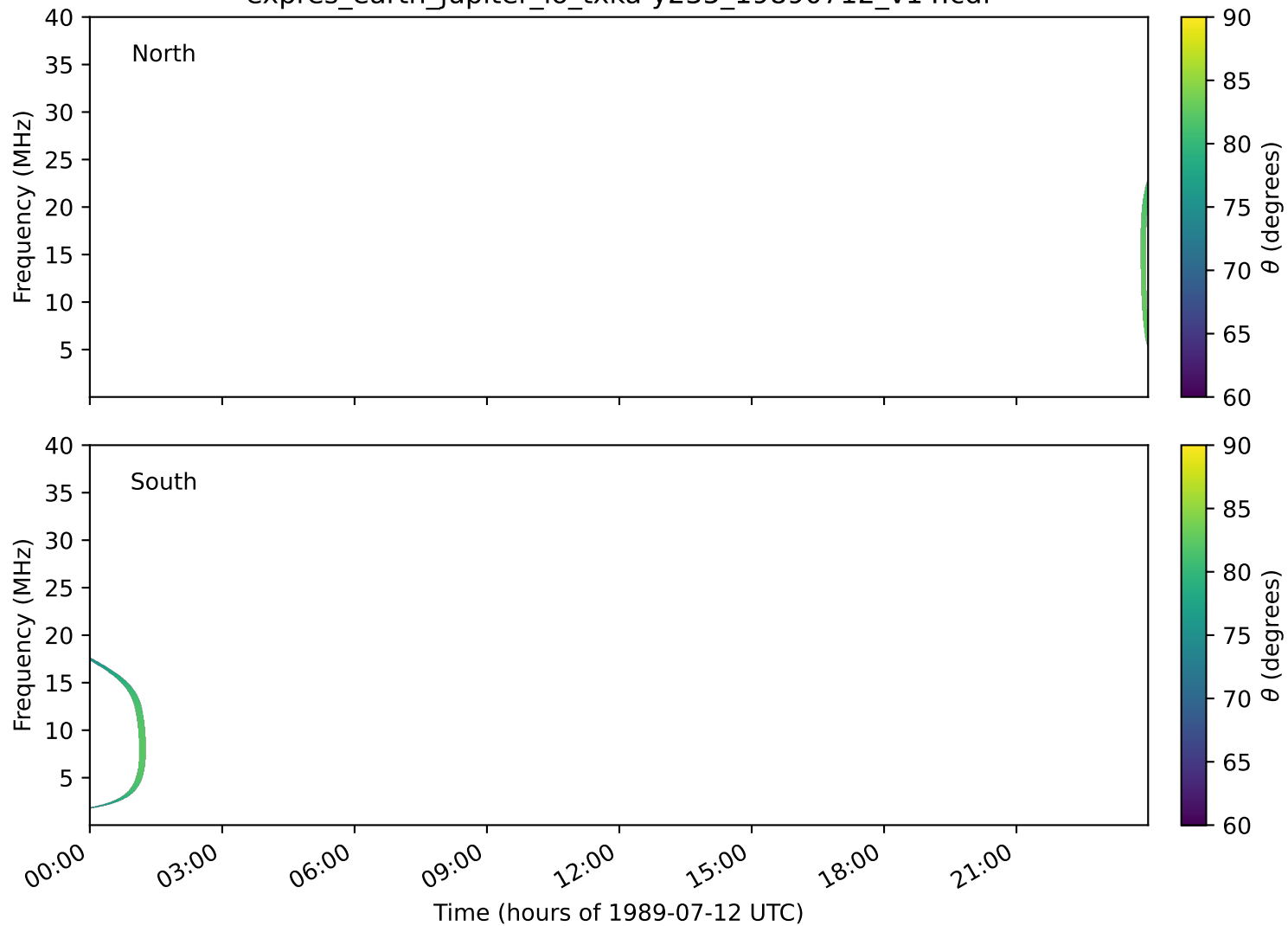
expres_earth_jupiter_io_txka-y235_19890712_v14.cdf
