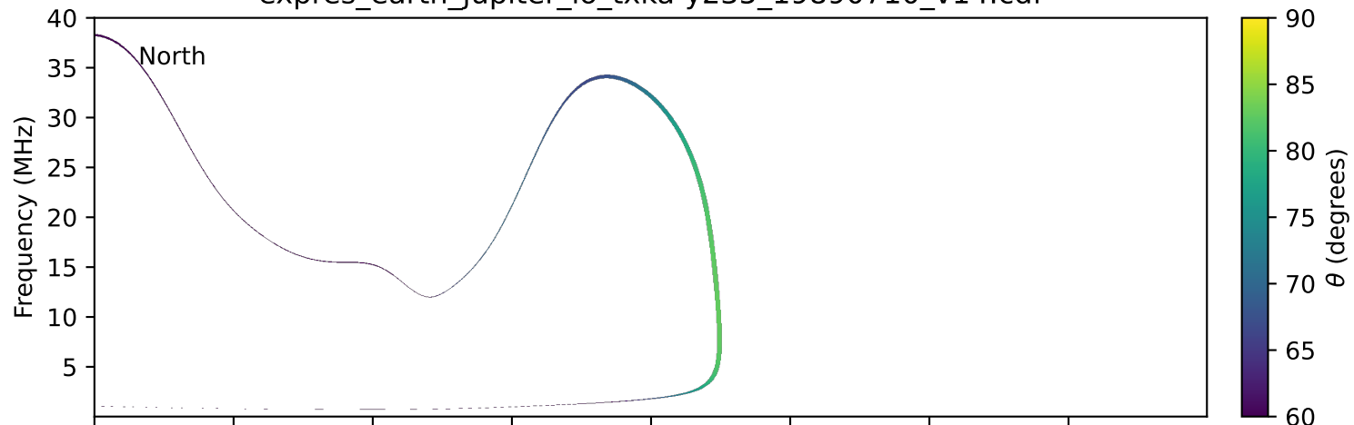
expres_earth_jupiter_io_txka-y235_19890710_v14.cdf
