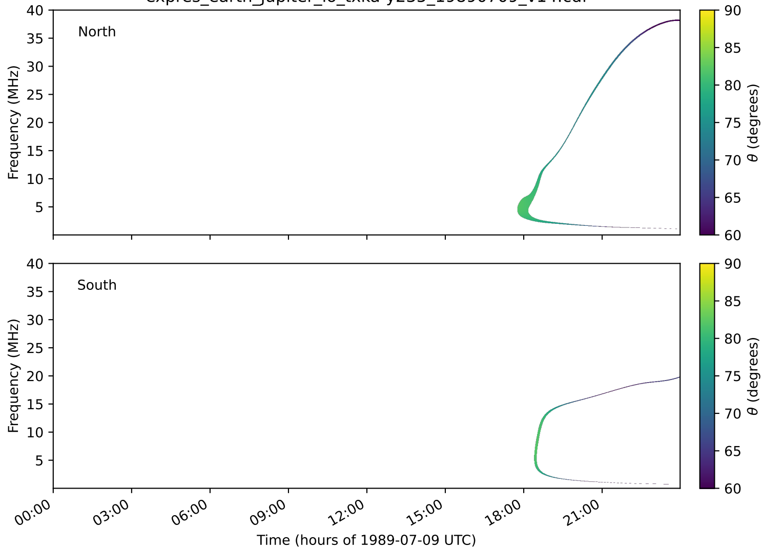
expres_earth_jupiter_io_txka-y235_19890709_v14.cdf
