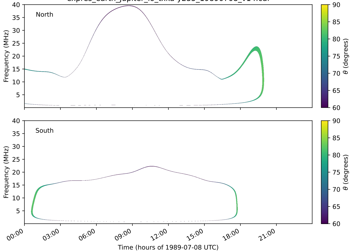
expres_earth_jupiter_io_txka-y235_19890708_v14.cdf
