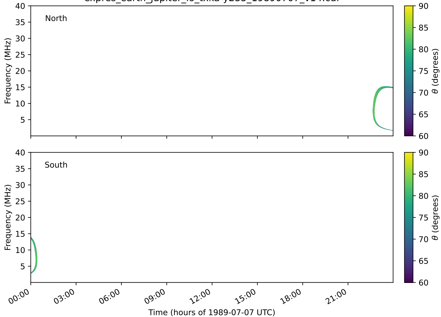
expres_earth_jupiter_io_txka-y235_19890707_v14.cdf
