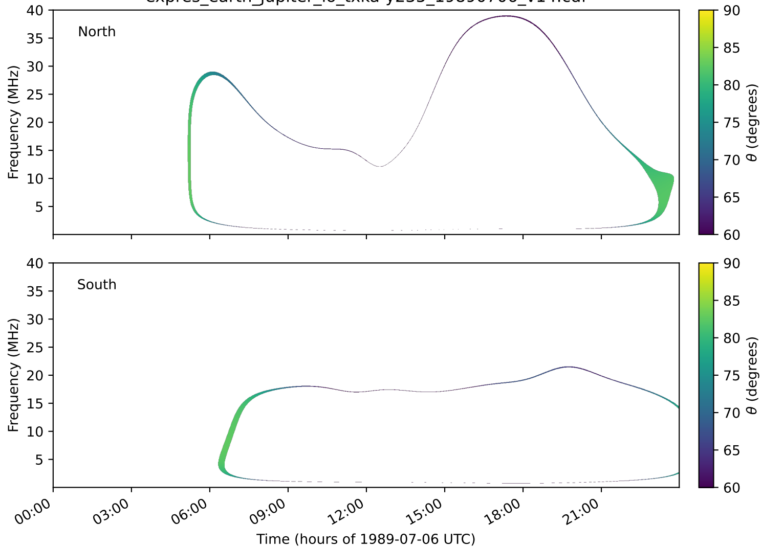
expres_earth_jupiter_io_txka-y235_19890706_v14.cdf
