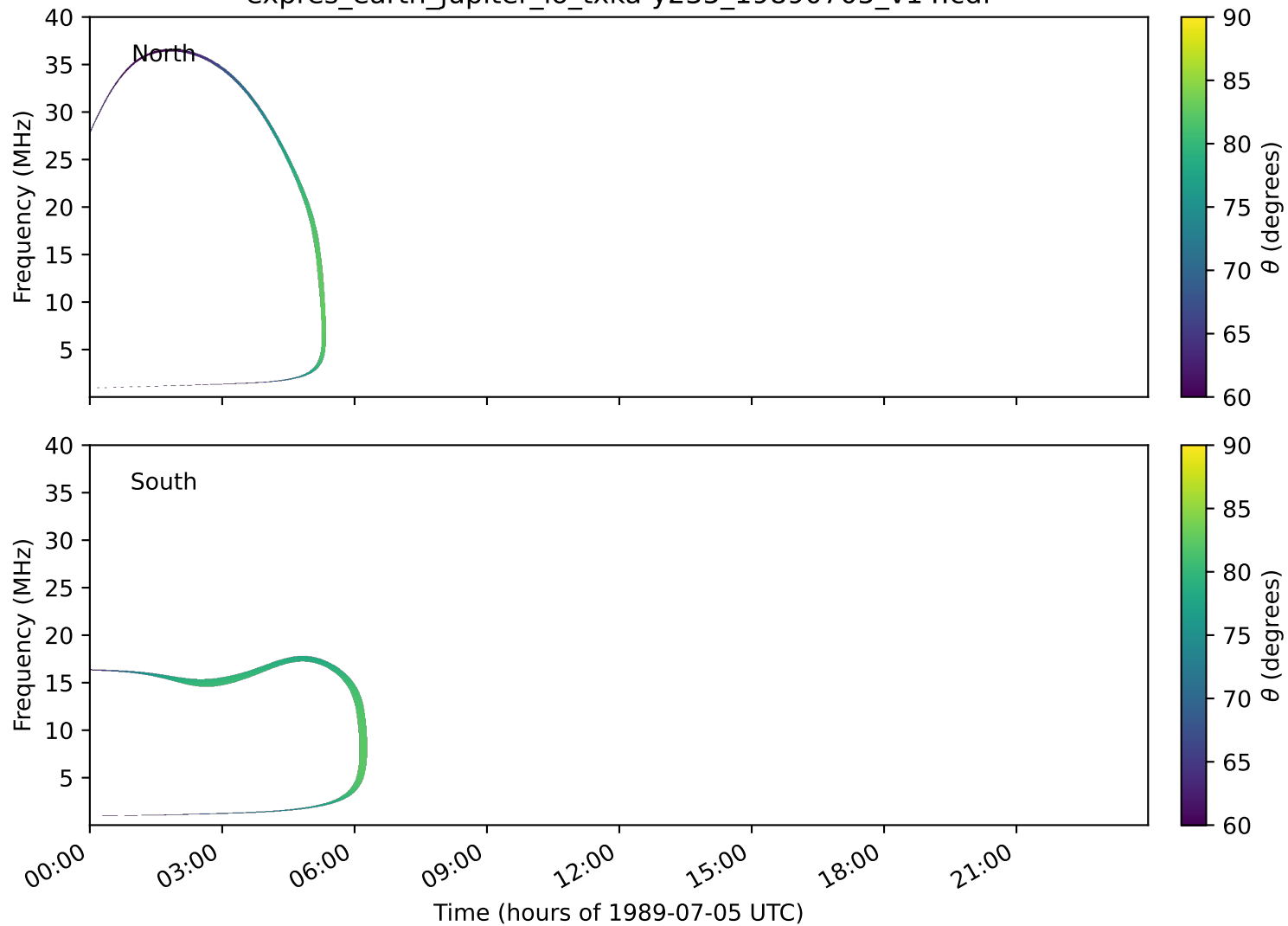
expres_earth_jupiter_io_txka-y235_19890705_v14.cdf
