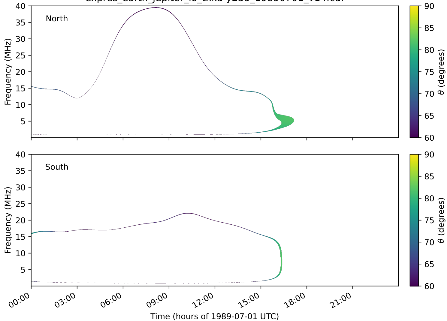
expres_earth_jupiter_io_txka-y235_19890701_v14.cdf
