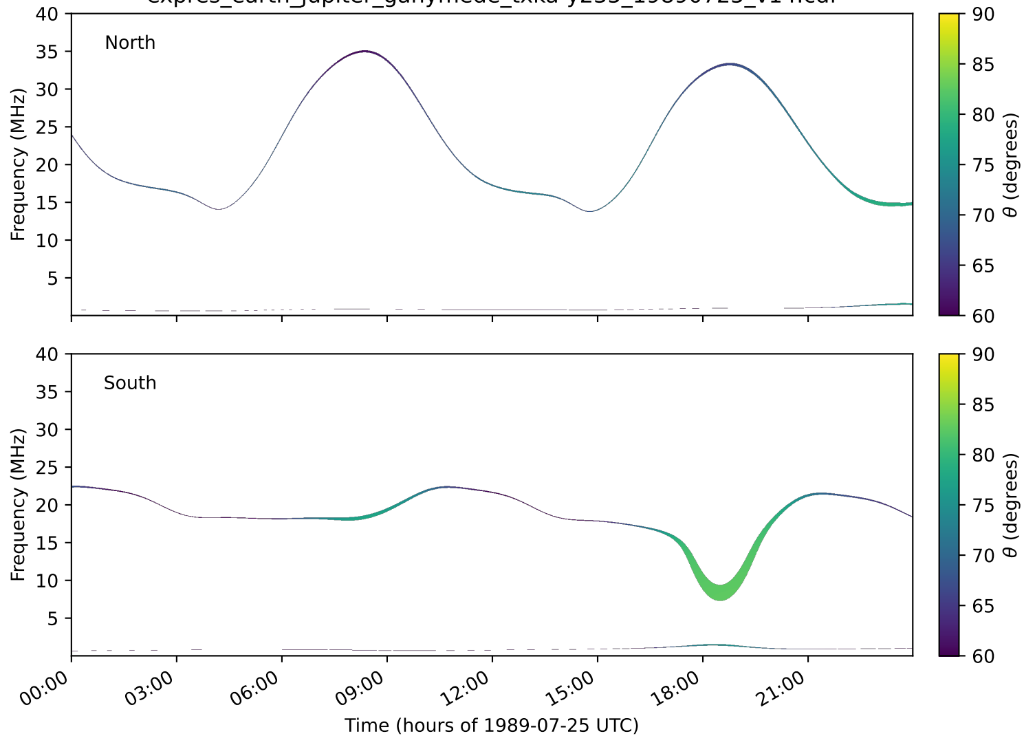
expres_earth_jupiter_ganymede_txka-y235_19890725_v14.cdf
