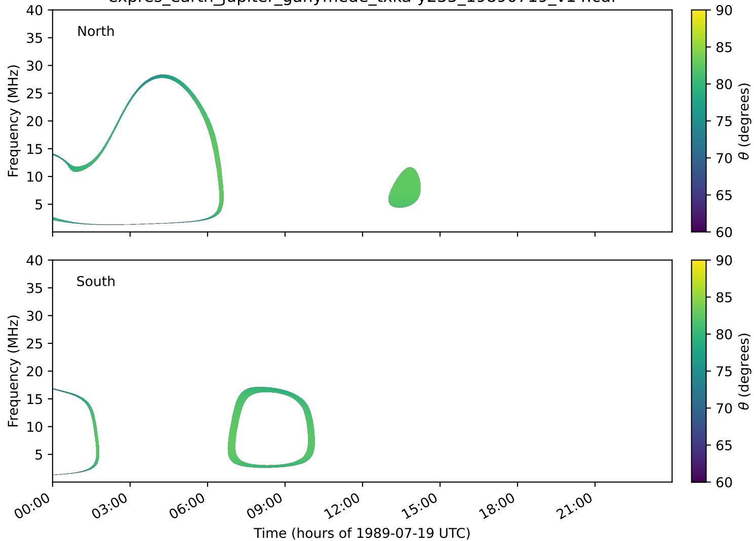
expres_earth_jupiter_ganymede_txka-y235_19890719_v14.cdf
