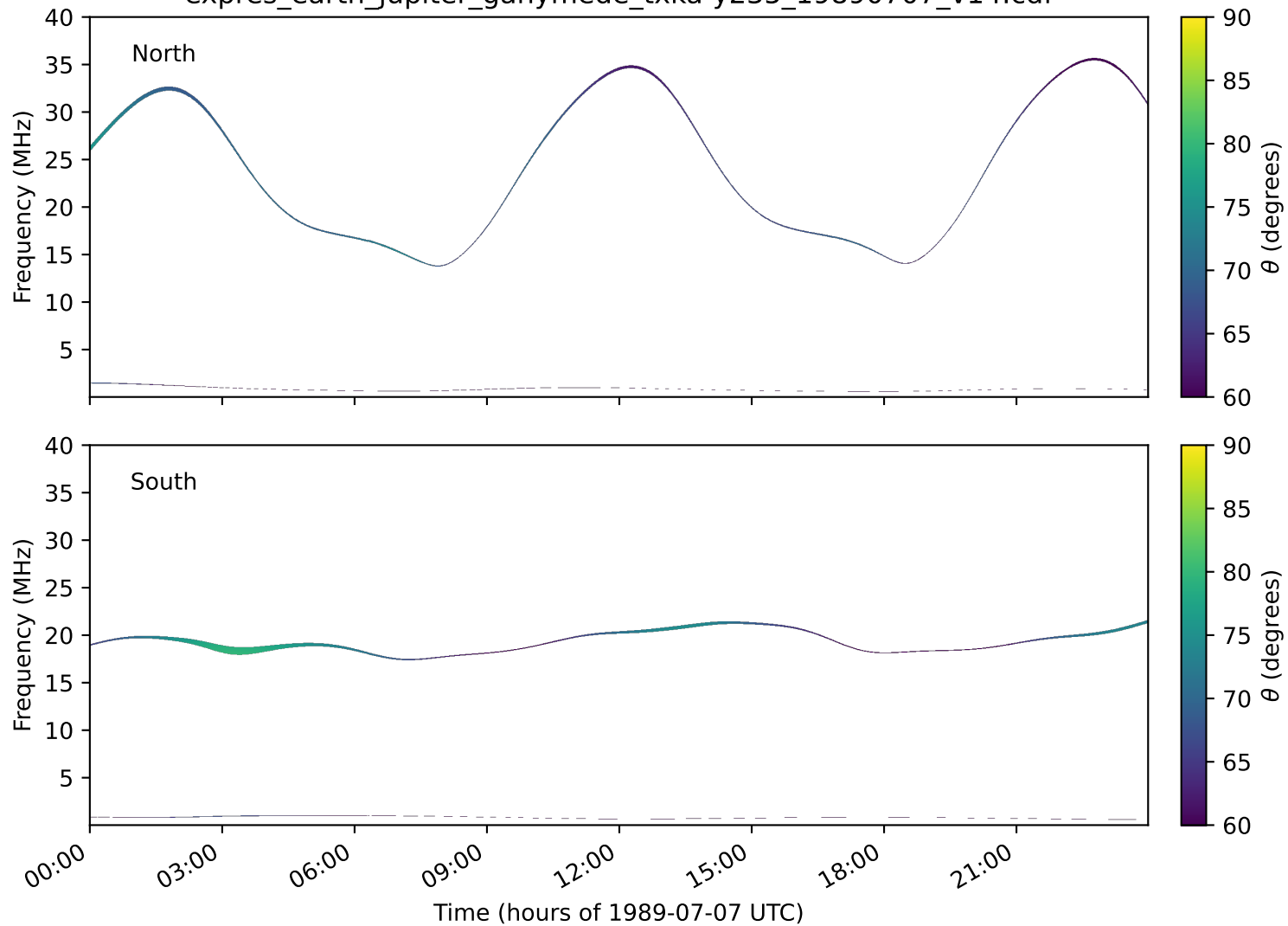
expres_earth_jupiter_ganymede_txka-y235_19890707_v14.cdf
