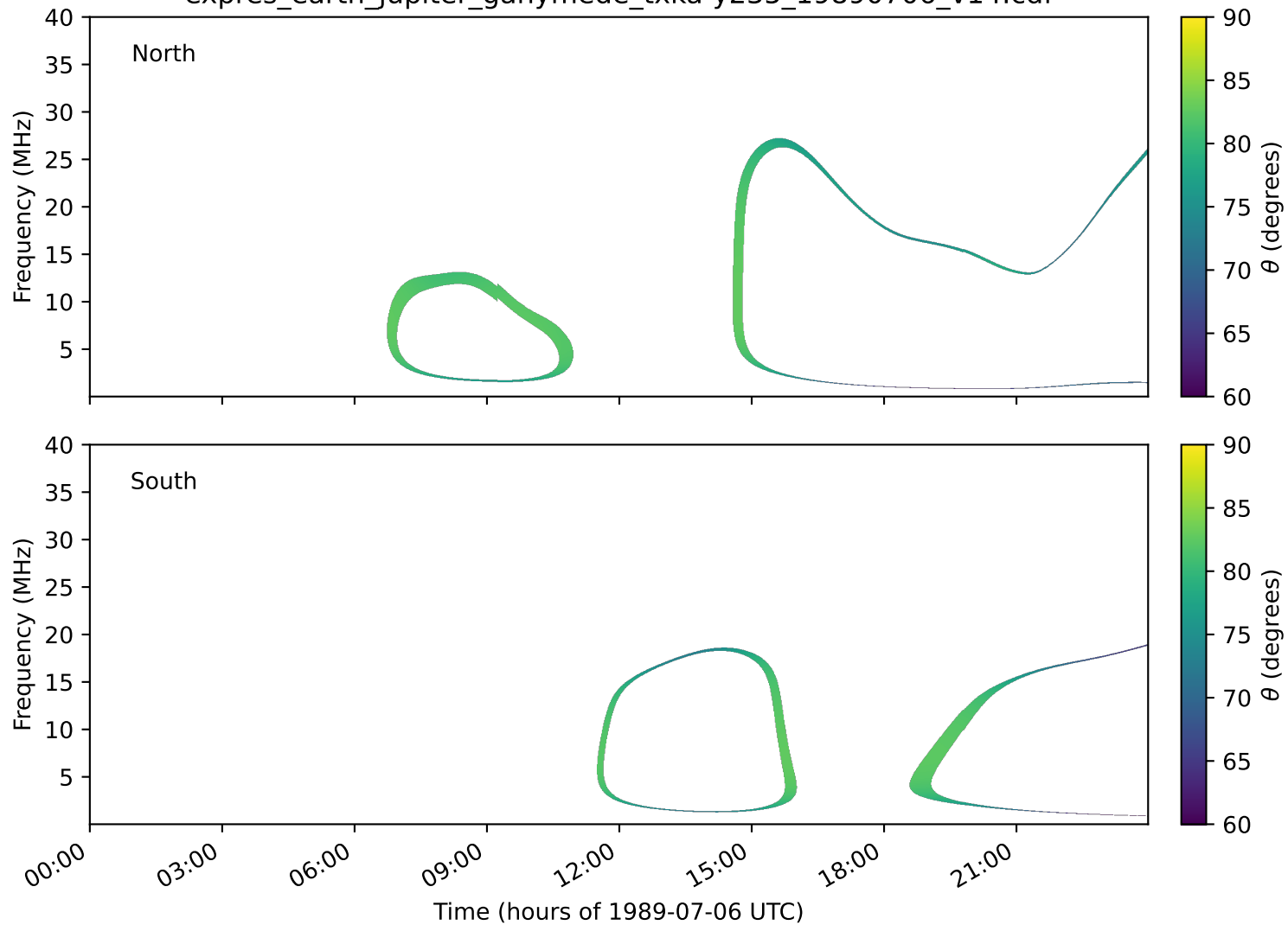
expres_earth_jupiter_ganymede_txka-y235_19890706_v14.cdf
