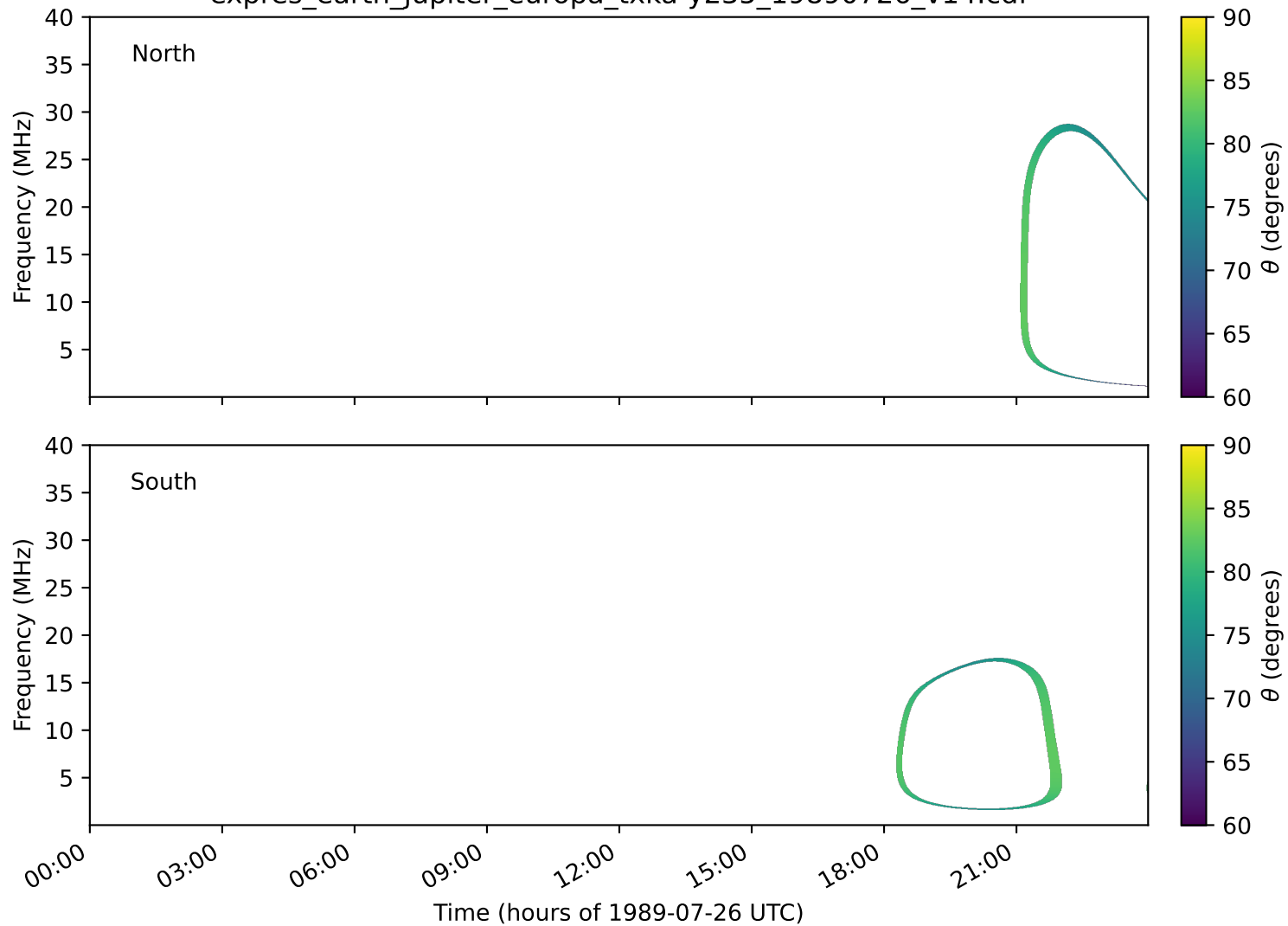
expres_earth_jupiter_europa_txka-y235_19890726_v14.cdf
