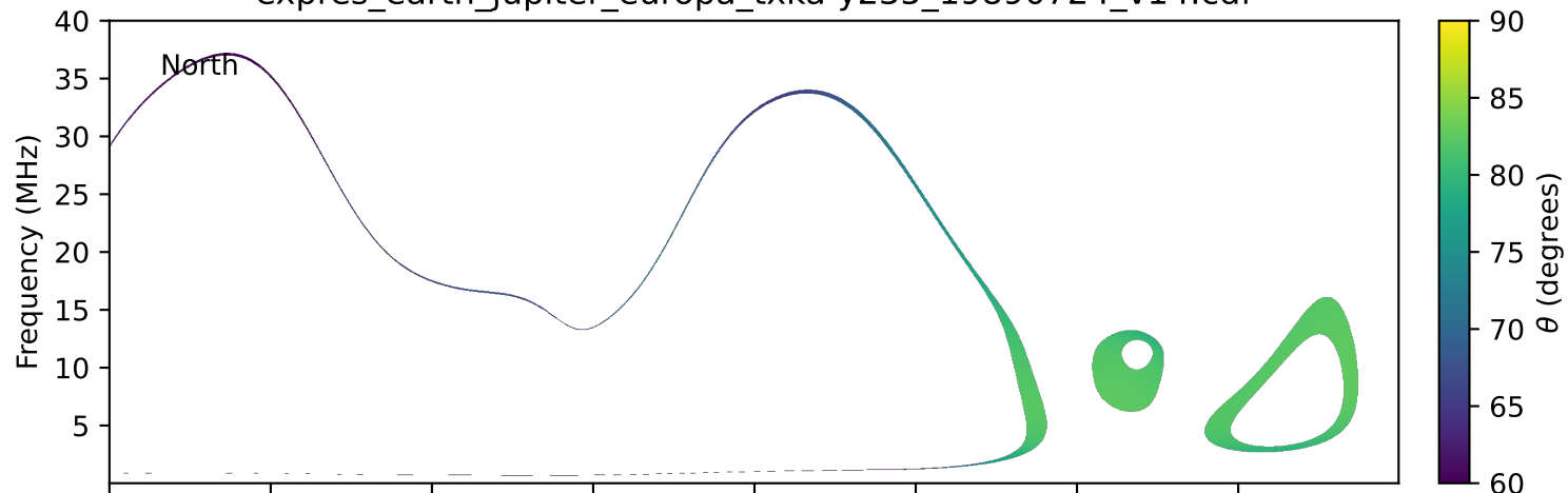
expres_earth_jupiter_europa_txka-y235_19890724_v14.cdf
