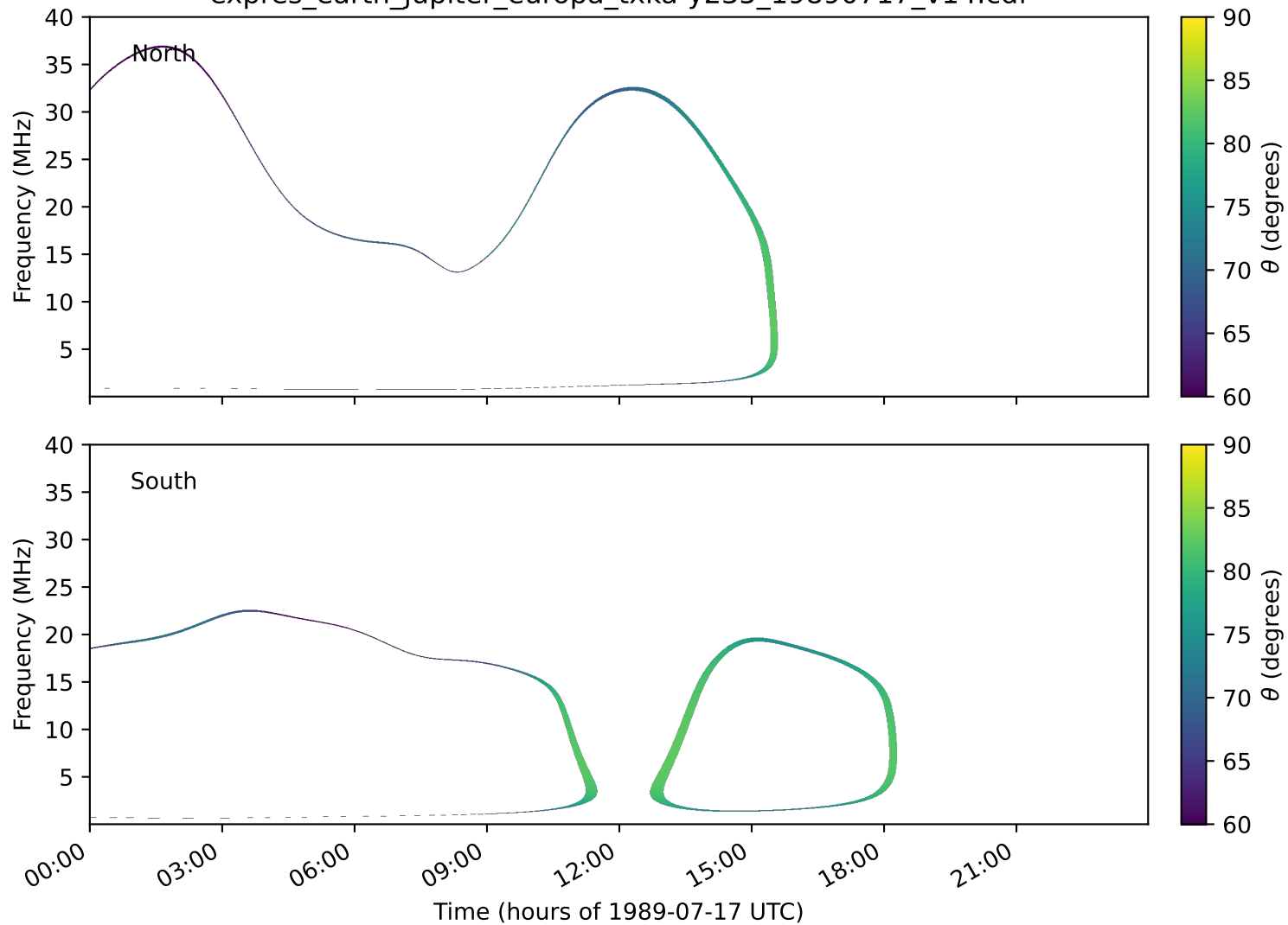
expres_earth_jupiter_europa_txka-y235_19890717_v14.cdf
