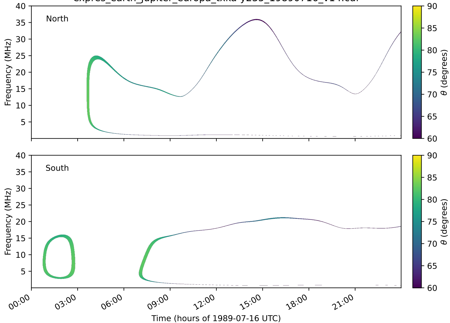
expres_earth_jupiter_europa_txka-y235_19890716_v14.cdf
