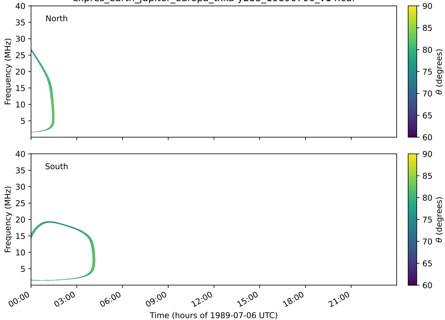
expres_earth_jupiter_europa_txka-y235_19890706_v14.cdf
