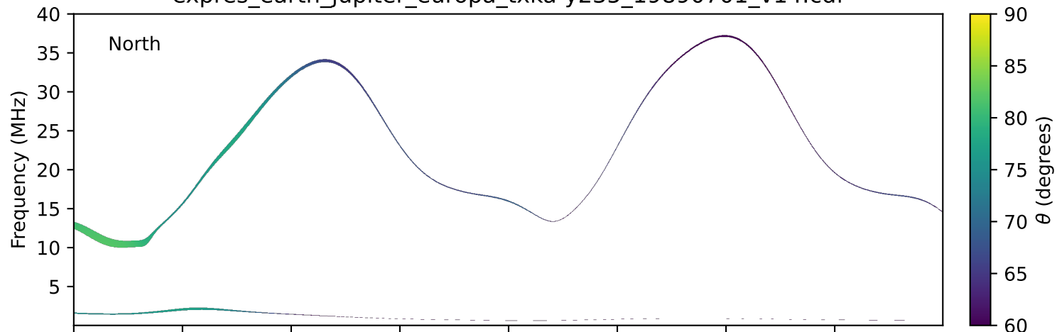
expres_earth_jupiter_europa_txka-y235_19890701_v14.cdf
