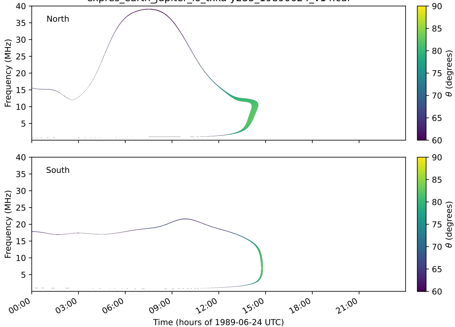
expres_earth_jupiter_io_txka-y235_19890624_v14.cdf
