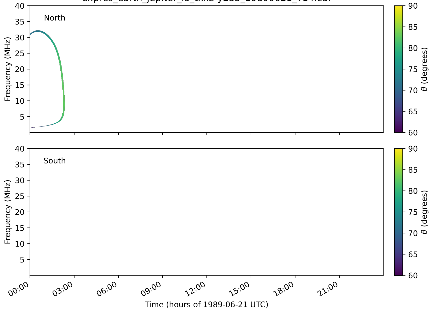
expres_earth_jupiter_io_txka-y235_19890621_v14.cdf
