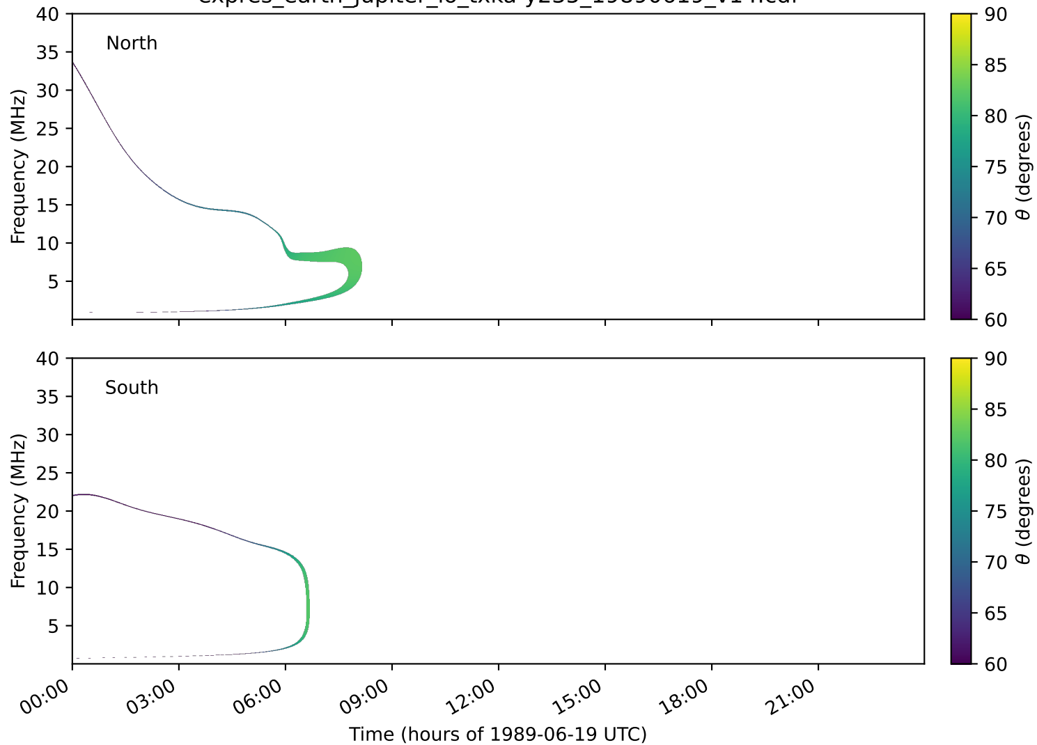
expres_earth_jupiter_io_txka-y235_19890619_v14.cdf
