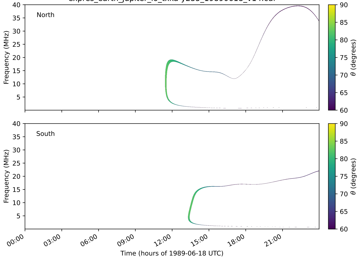
expres_earth_jupiter_io_txka-y235_19890618_v14.cdf
