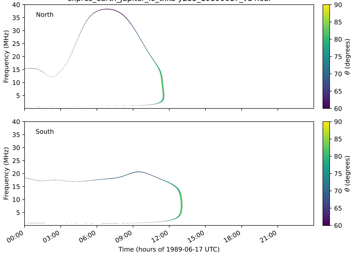
expres_earth_jupiter_io_txka-y235_19890617_v14.cdf
