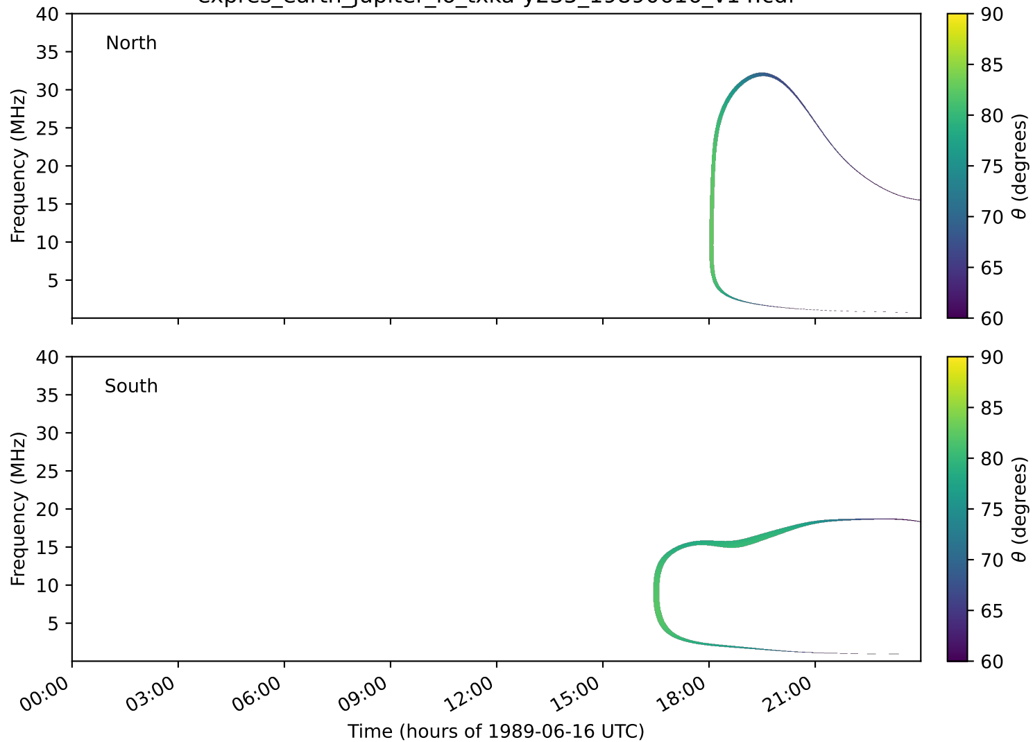
expres_earth_jupiter_io_txka-y235_19890616_v14.cdf
