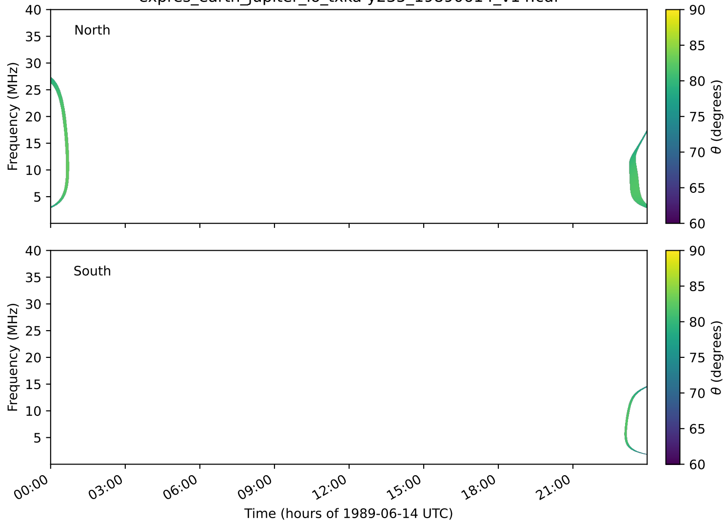
expres_earth_jupiter_io_txka-y235_19890614_v14.cdf
