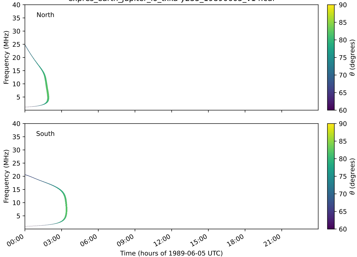
expres_earth_jupiter_io_txka-y235_19890605_v14.cdf
