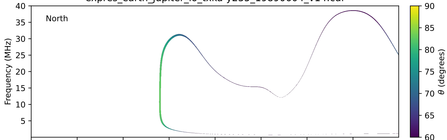
expres_earth_jupiter_io_txka-y235_19890604_v14.cdf
