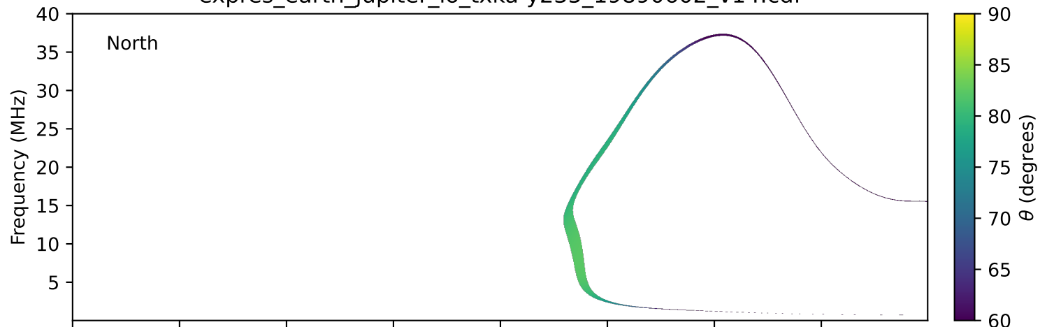
expres_earth_jupiter_io_txka-y235_19890602_v14.cdf
