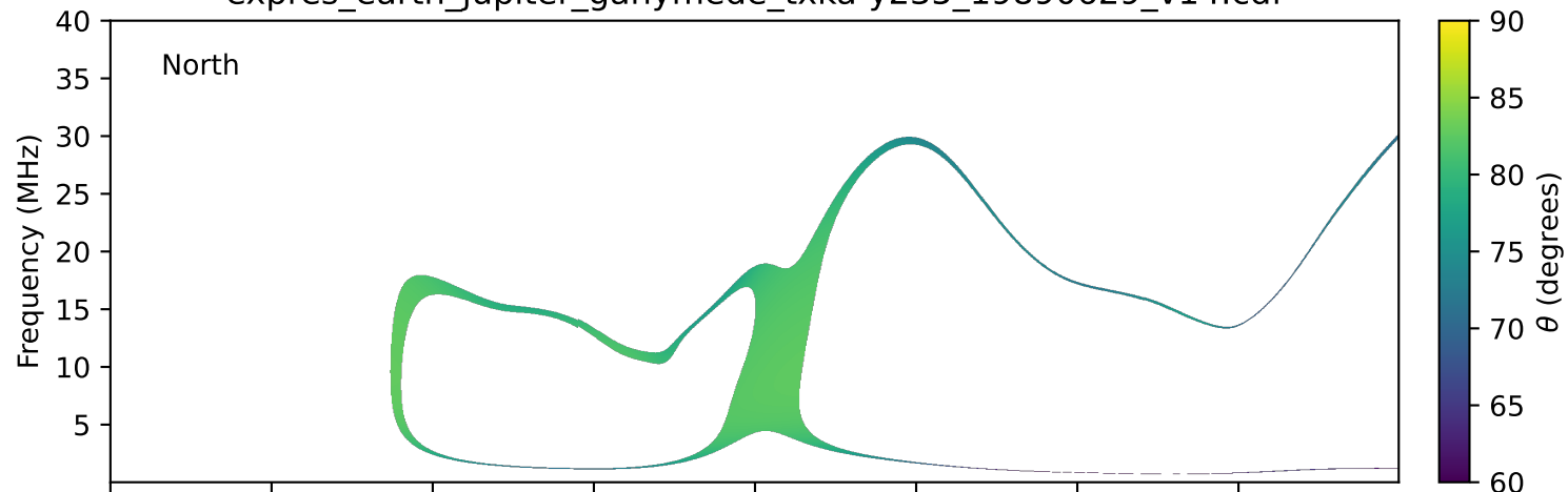
expres_earth_jupiter_ganymede_txka-y235_19890629_v14.cdf
