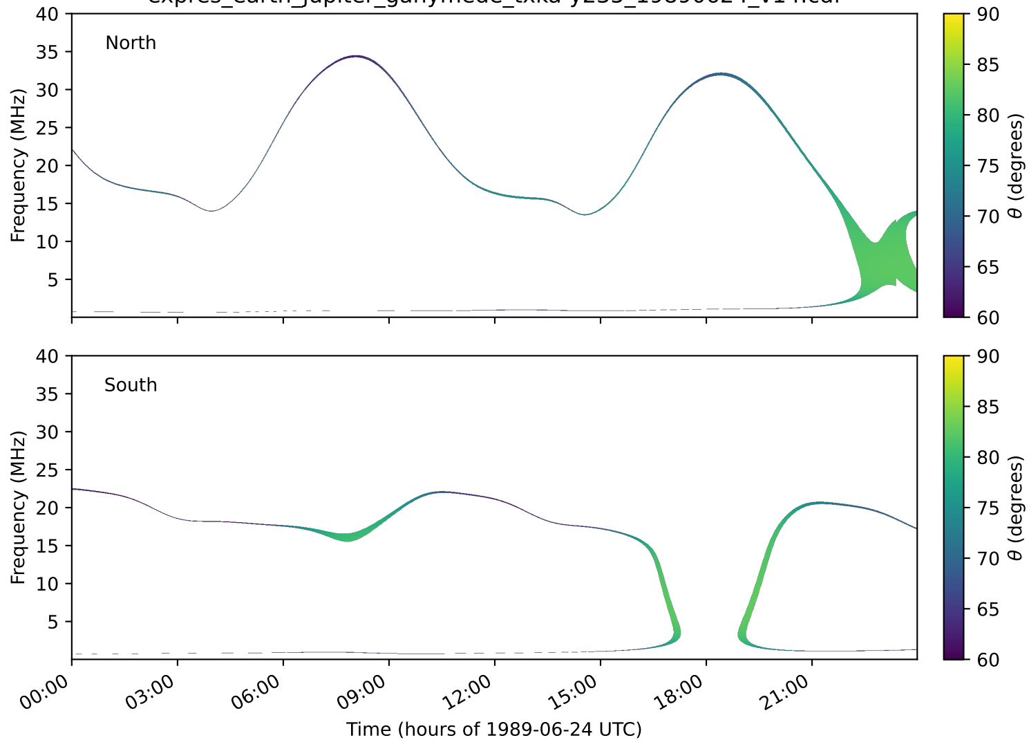
expres_earth_jupiter_ganymede_txka-y235_19890624_v14.cdf
