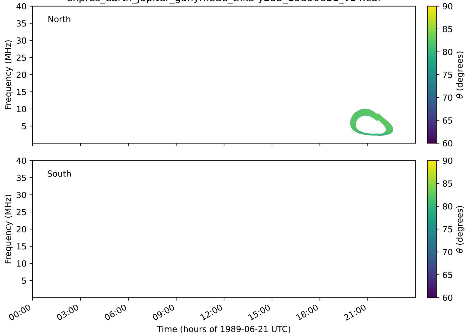
expres_earth_jupiter_ganymede_txka-y235_19890621_v14.cdf
