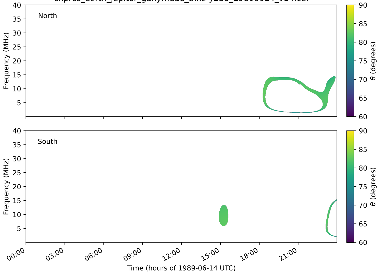
expres_earth_jupiter_ganymede_txka-y235_19890614_v14.cdf
