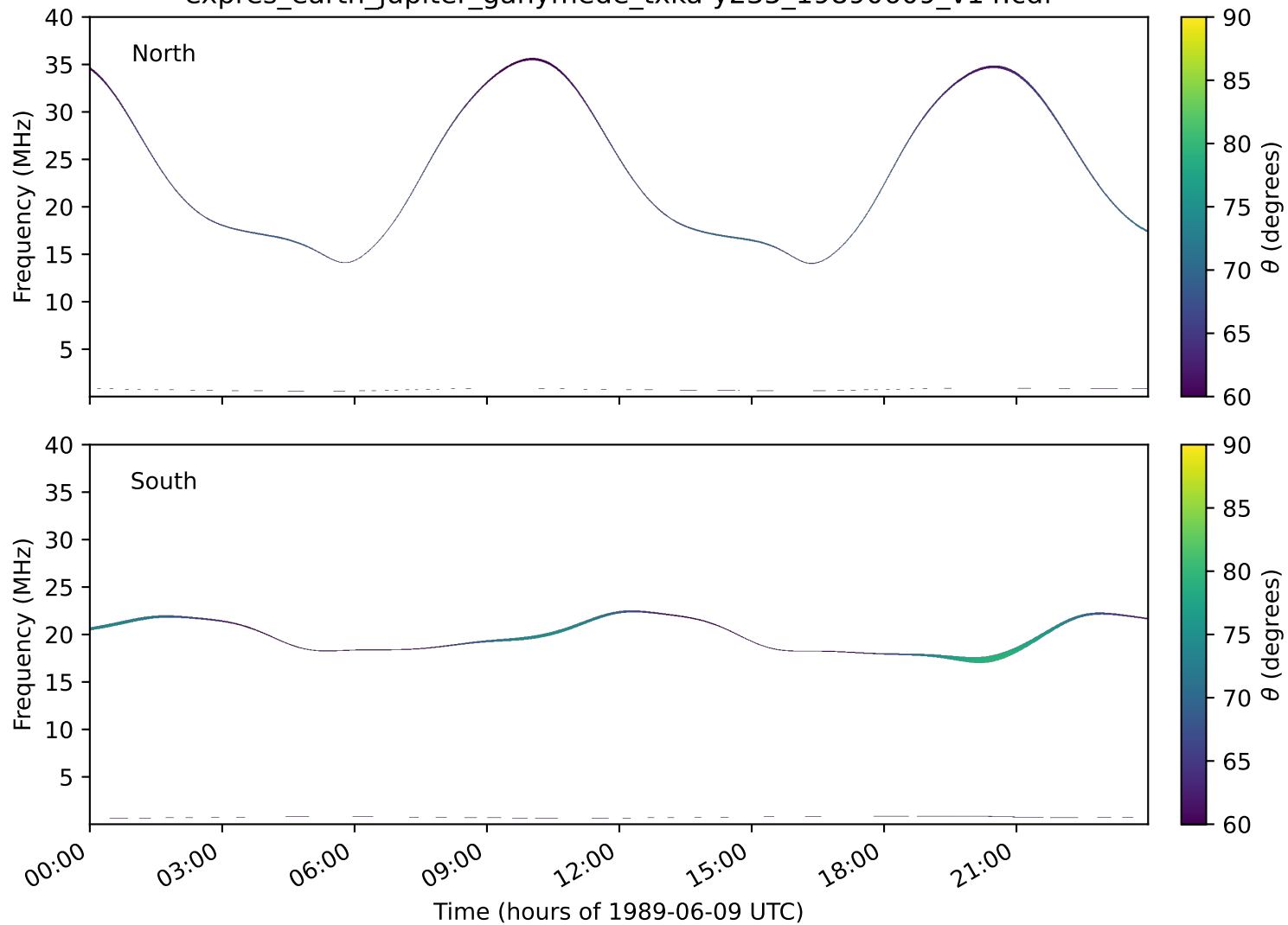
expres_earth_jupiter_ganymede_txka-y235_19890609_v14.cdf
