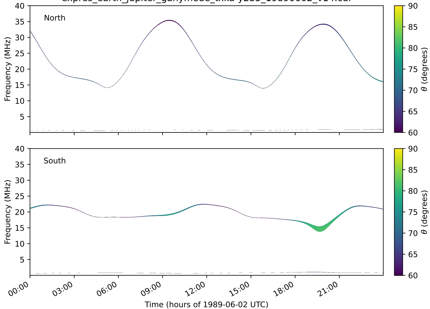
expres_earth_jupiter_ganymede_txka-y235_19890602_v14.cdf
