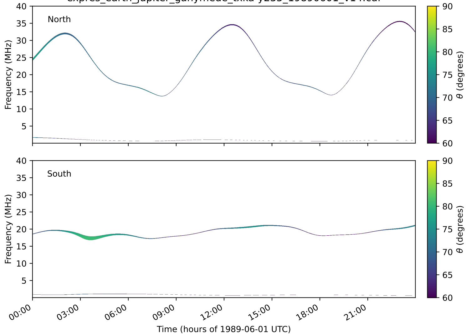
expres_earth_jupiter_ganymede_txka-y235_19890601_v14.cdf
