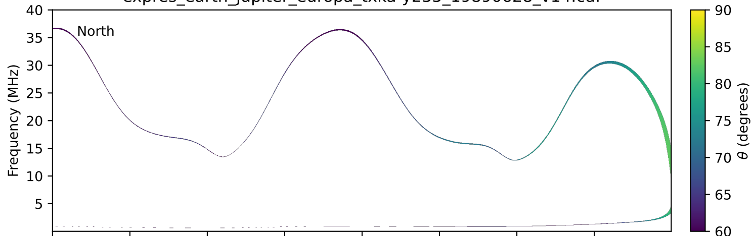
expres_earth_jupiter_europa_txka-y235_19890628_v14.cdf
