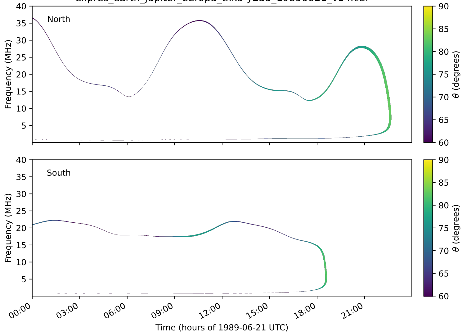
expres_earth_jupiter_europa_txka-y235_19890621_v14.cdf
