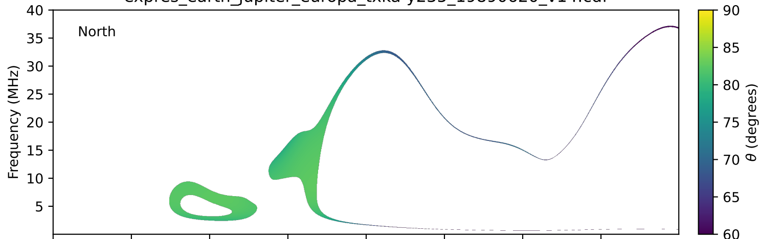
expres_earth_jupiter_europa_txka-y235_19890620_v14.cdf
