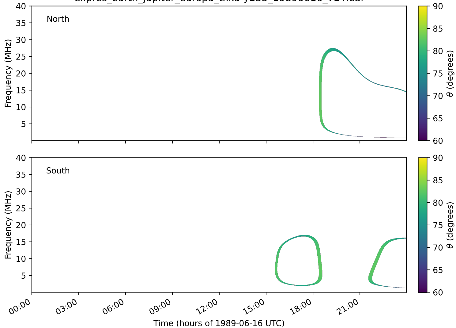
expres_earth_jupiter_europa_txka-y235_19890616_v14.cdf
