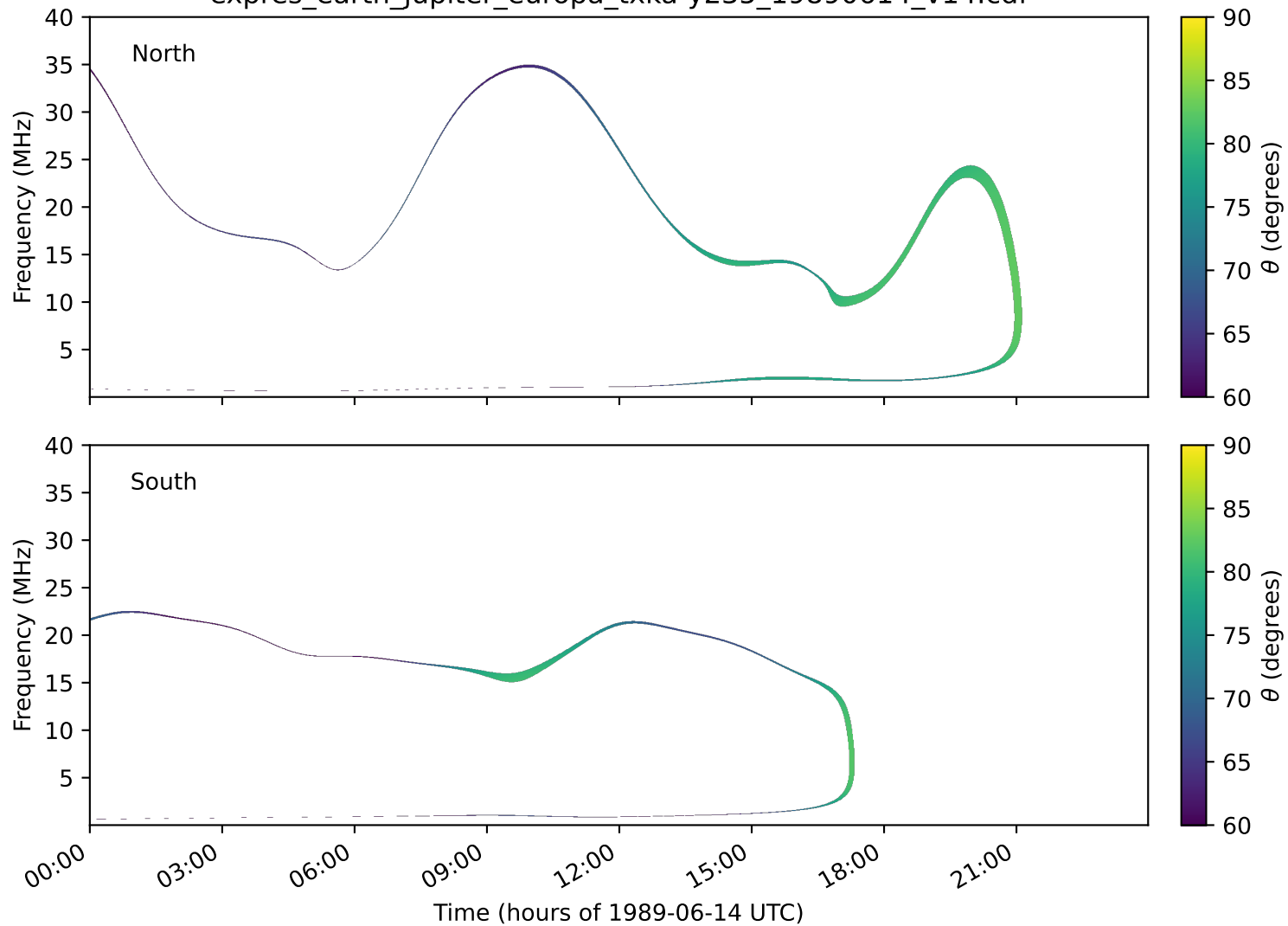
expres_earth_jupiter_europa_txka-y235_19890614_v14.cdf
