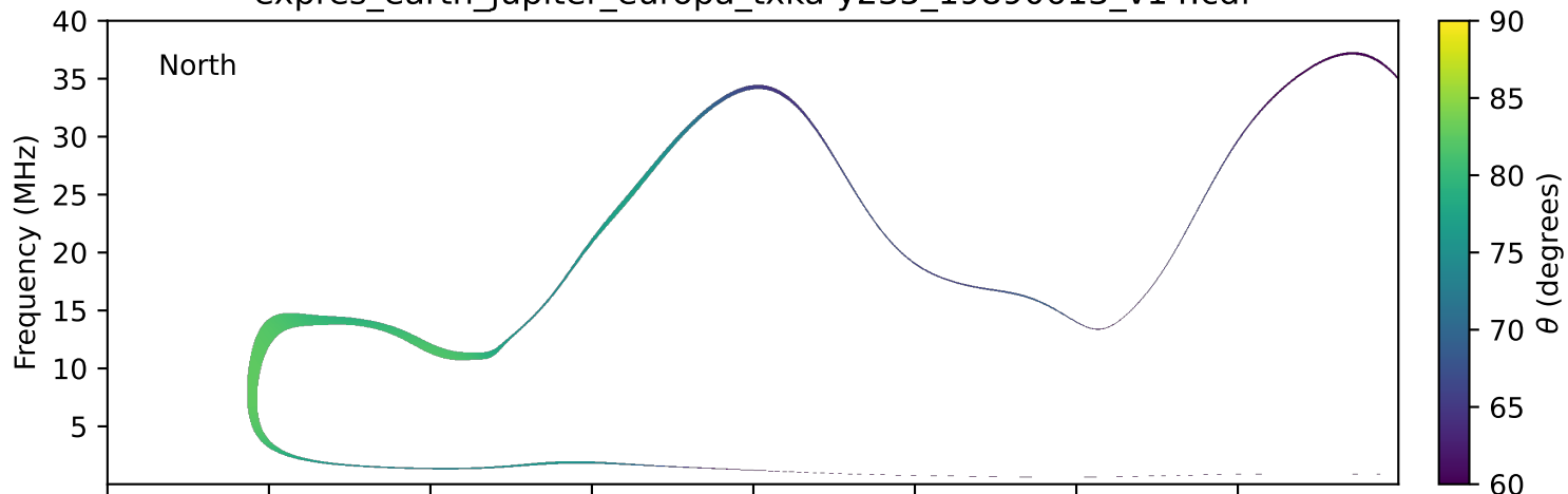
expres_earth_jupiter_europa_txka-y235_19890613_v14.cdf
