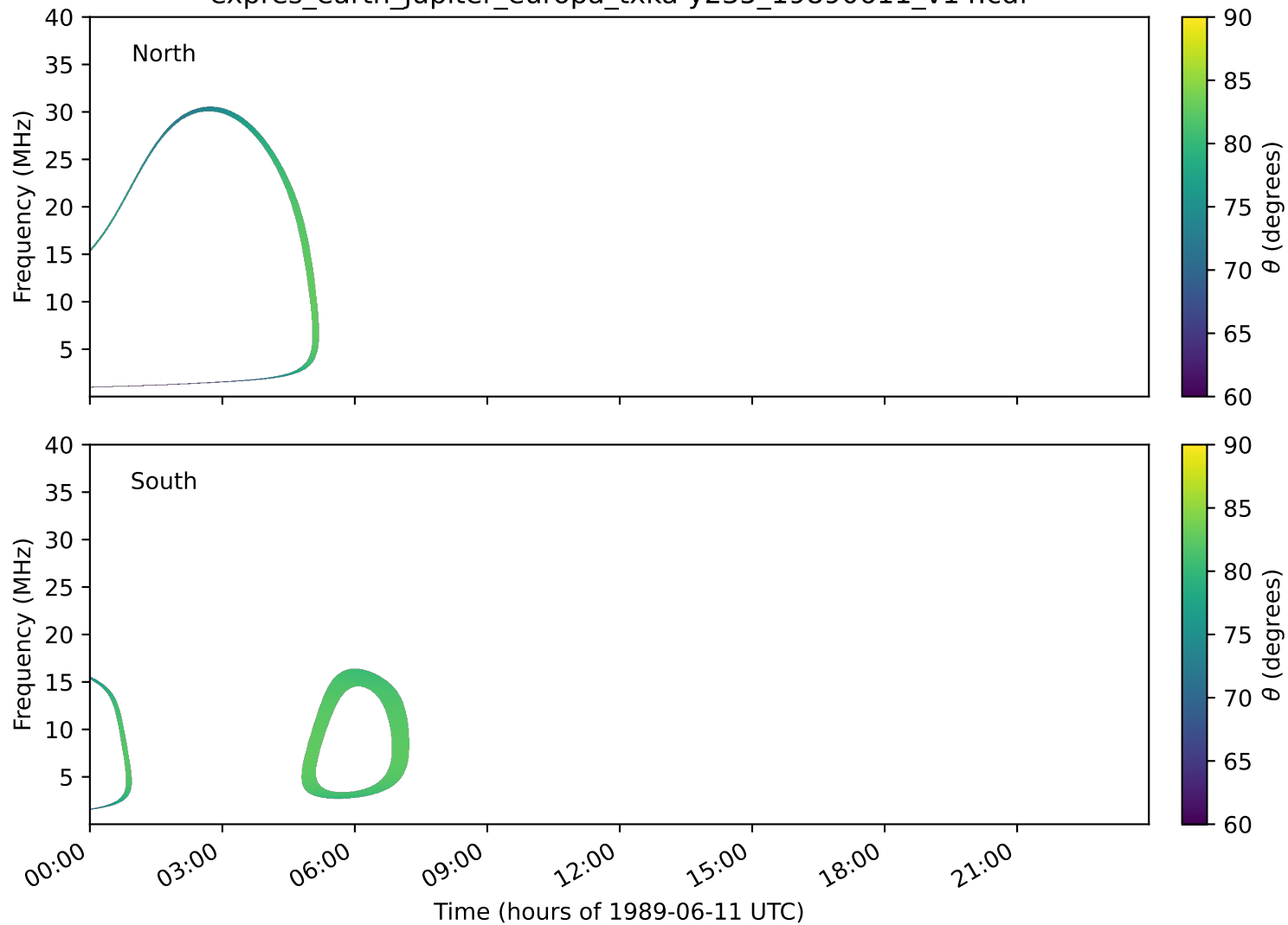
expres_earth_jupiter_europa_txka-y235_19890611_v14.cdf
