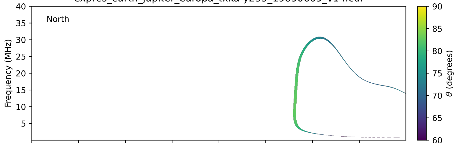
expres_earth_jupiter_europa_txka-y235_19890609_v14.cdf
