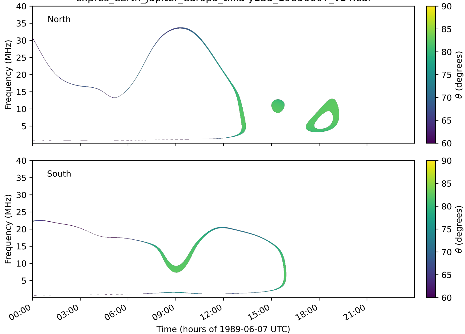
expres_earth_jupiter_europa_txka-y235_19890607_v14.cdf
