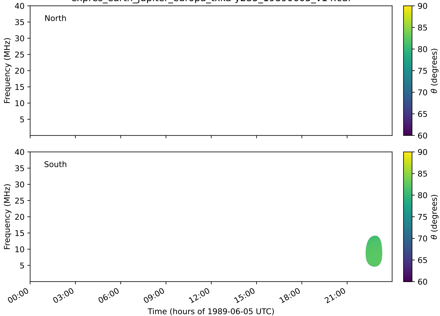
expres_earth_jupiter_europa_txka-y235_19890605_v14.cdf
