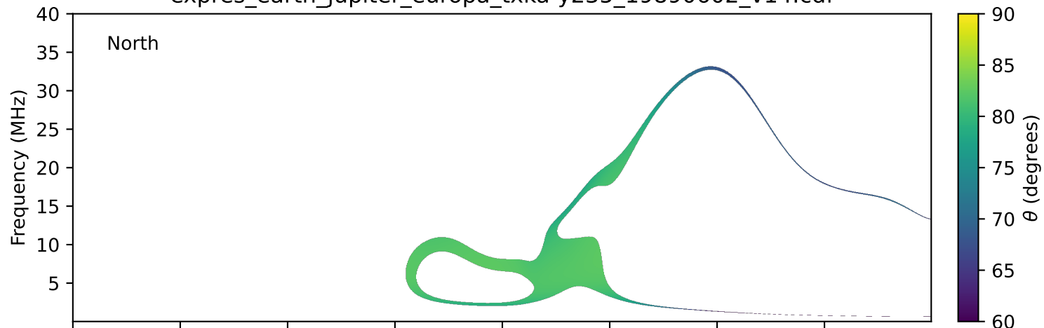
expres_earth_jupiter_europa_txka-y235_19890602_v14.cdf
